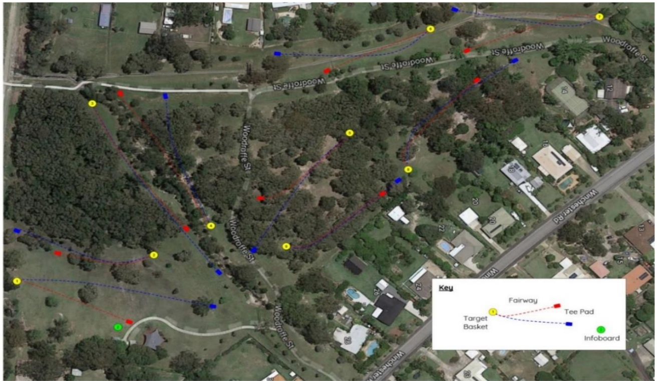
Meridan Downs Dual Tee 9 Target Course Design Layout
